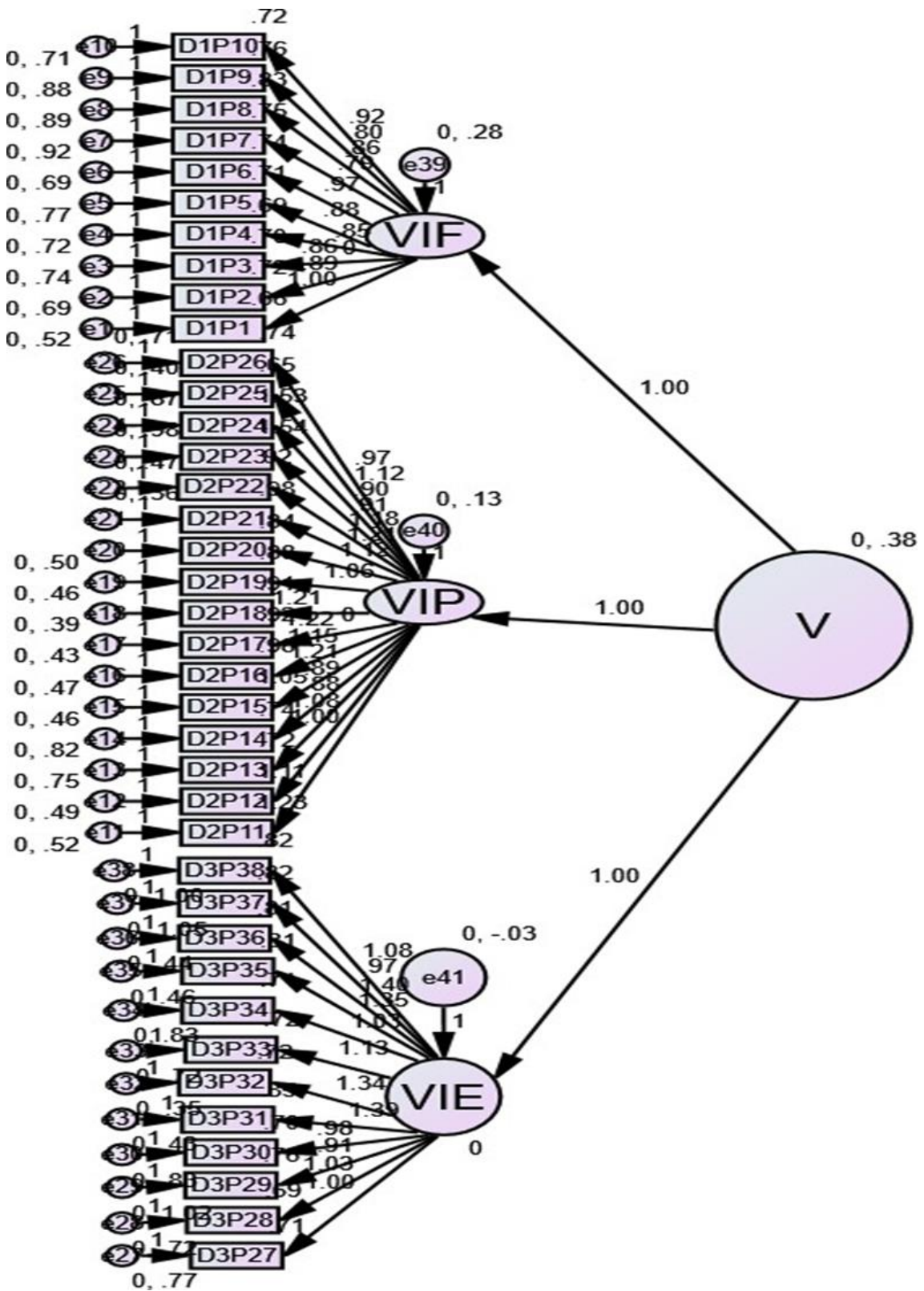
Path Diagram
